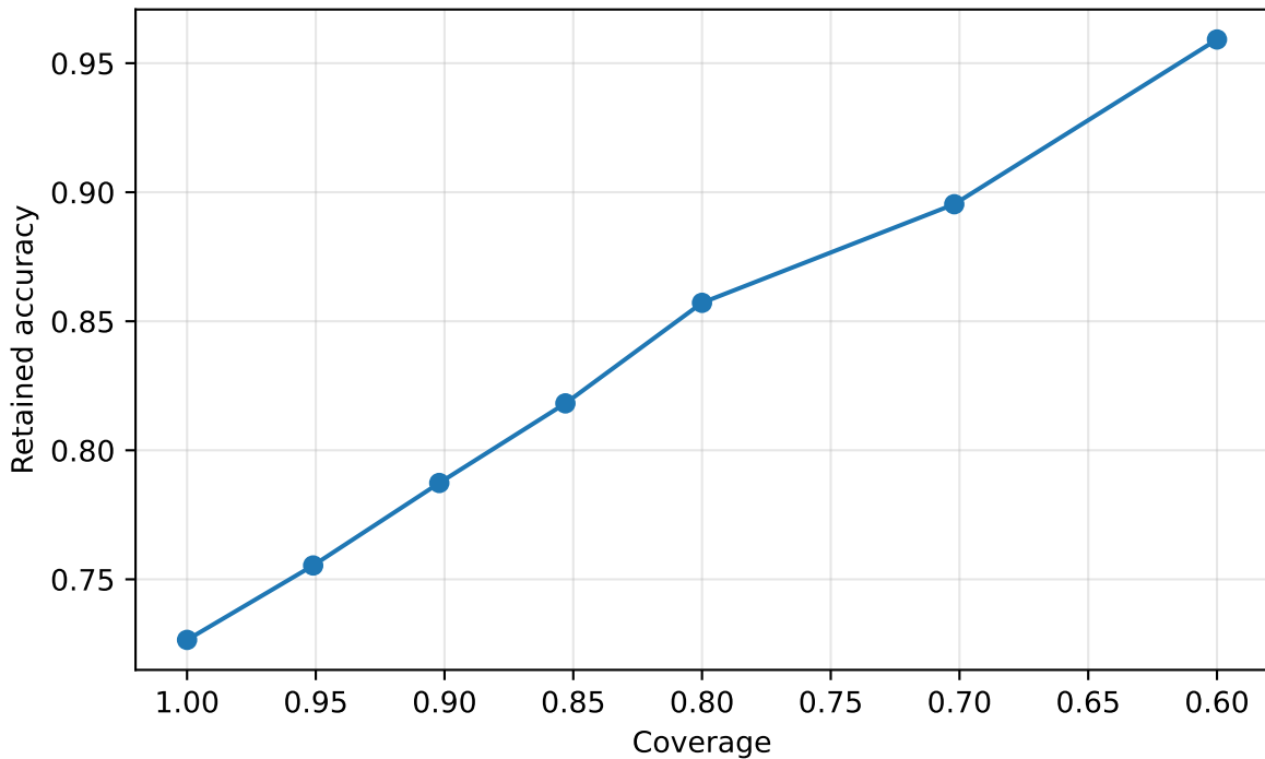
Retained accuracy vs coverage
