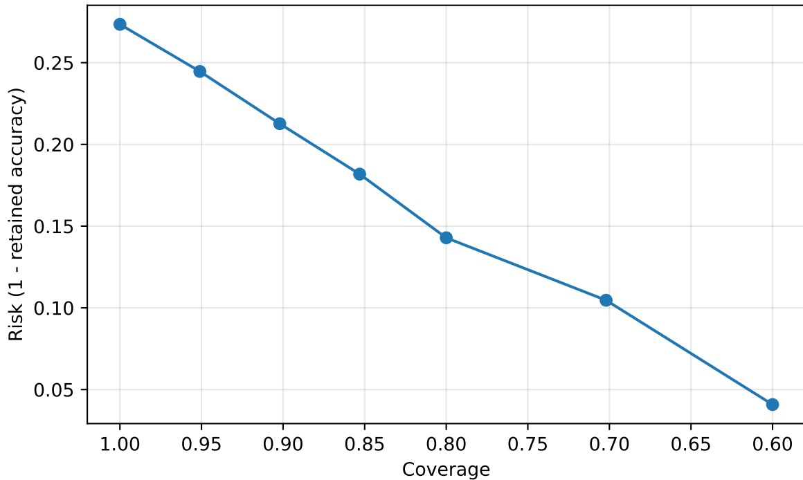
Risk-coverage curve
