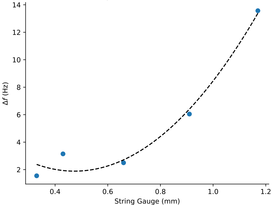
Inharmonicity Deviation on the 4th Harmonic
