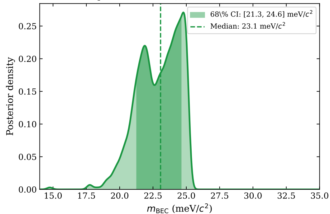
BEC particle mass: m_{\text{BEC}} = 23.1 \pm 1.6 \text{ meV}/c^2
