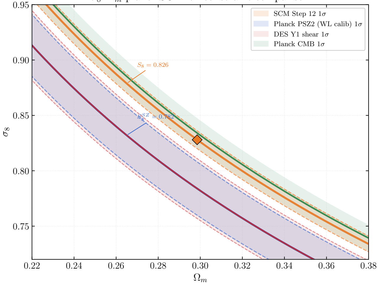
\sigma_8 - \Omega_m plane: SCM VI constraint comparison
