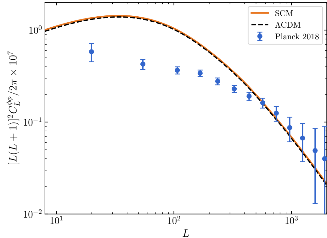
CMB lensing potential power spectrum
