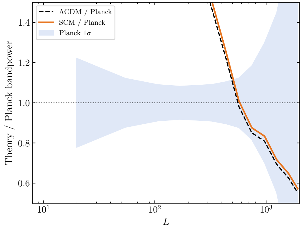
Ratio to Planck 2018
