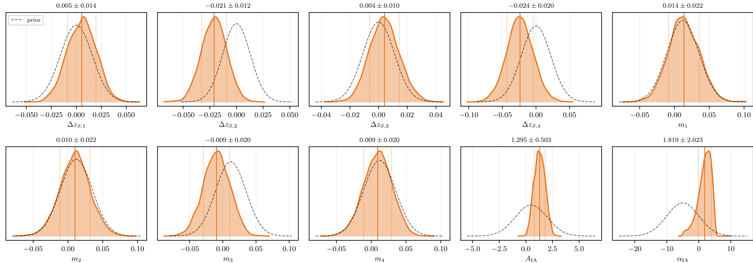
DES Y1 shear nuisance parameters: Step 12 posterior (orange) vs prior (dashed)
