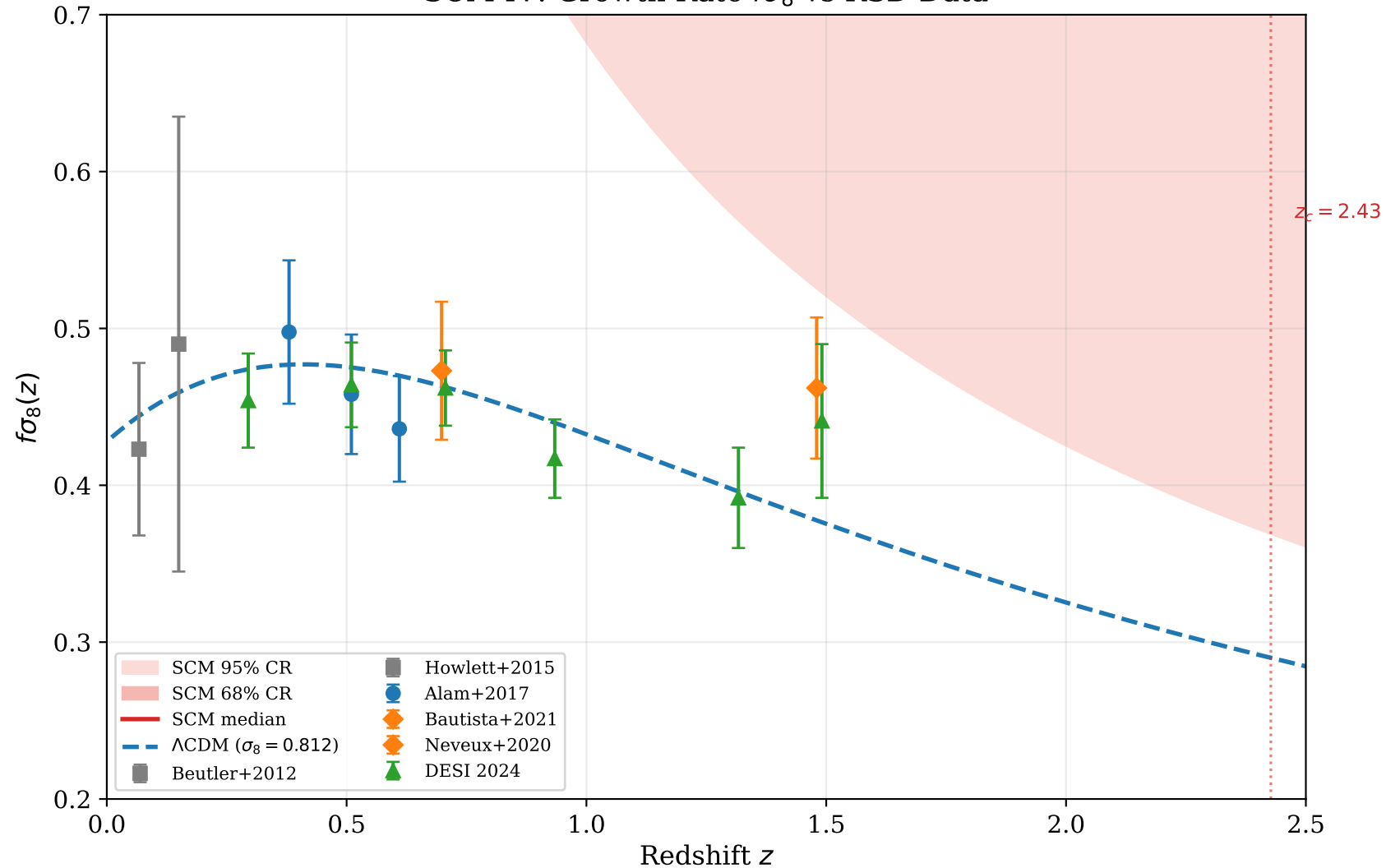
SCM IV: Growth Rate f\sigma_8 vs RSD Data
