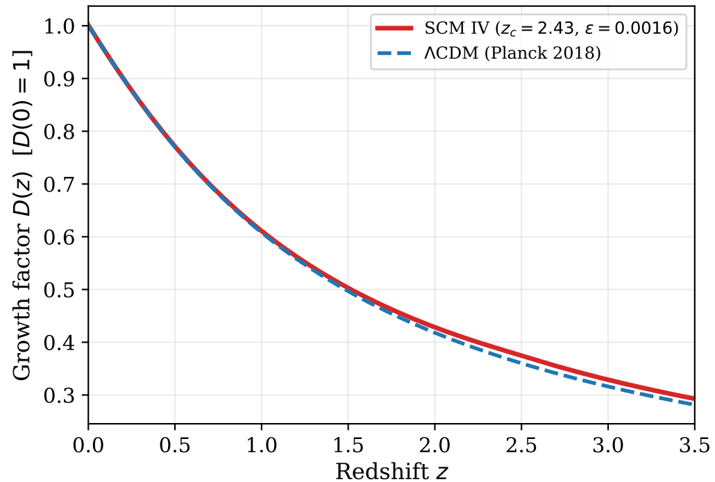
Linear Growth Factor
