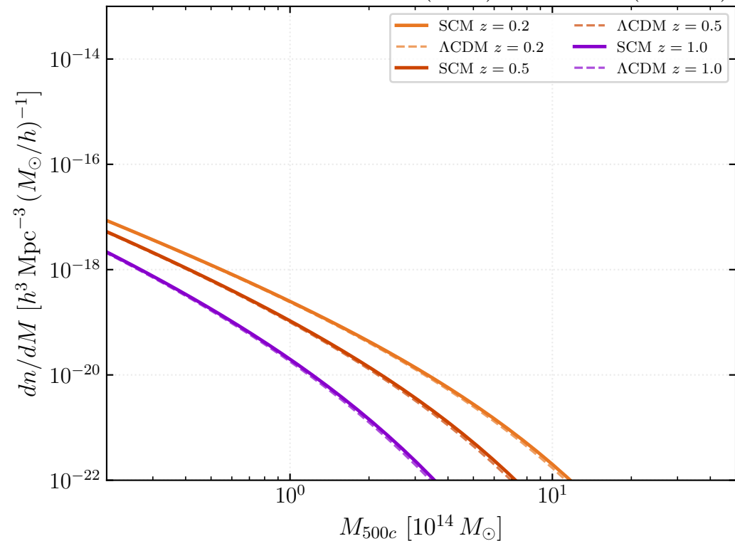
Halo mass function: SCM (solid) vs \Lambda CDM (dashed)
