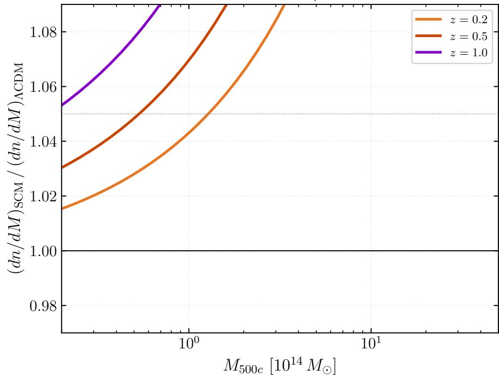
HMF ratio SCM/ \Lambda CDM
