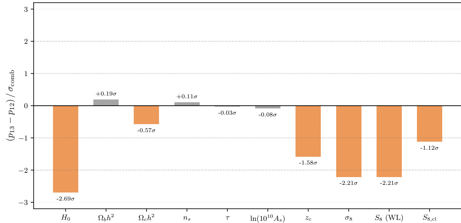
Parameter shifts Step 13 vs Step 12: effect of adding Planck SZ clusters
