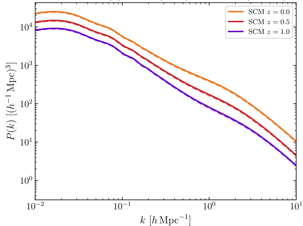
Non-linear P(k) : SCM (solid) vs \Lambda CDM (dashed)
