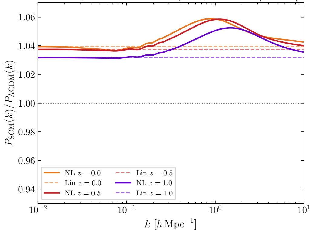
Power spectrum ratio: NL (solid) vs linear (dashed)
