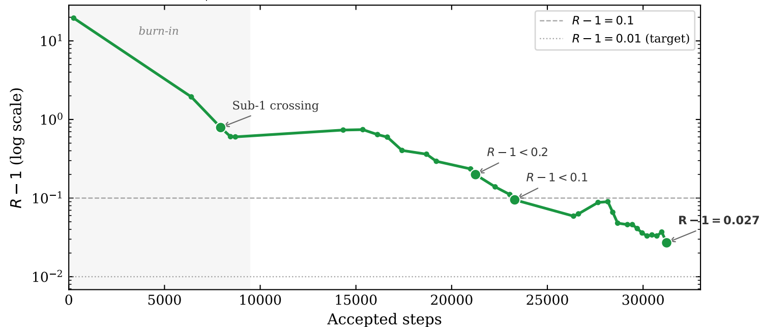
Step 10: R - 1 convergence trajectory ( \epsilon, A_{\text{fp}} ) parameterisation, z_{C, \text{max}} = 3.0 with prior rejection
