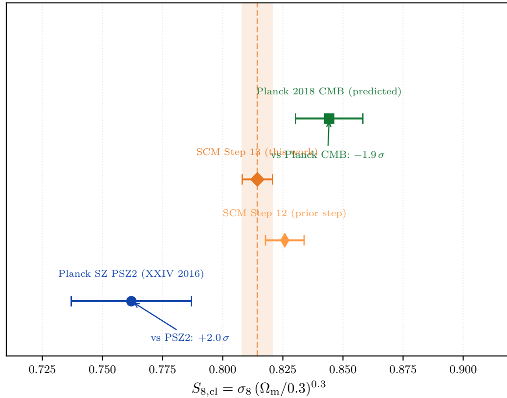
S_{8,\text{cl}} : cluster-count combination
