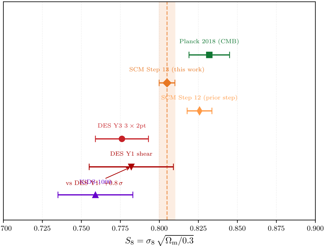
S_8 : weak-lensing combination
