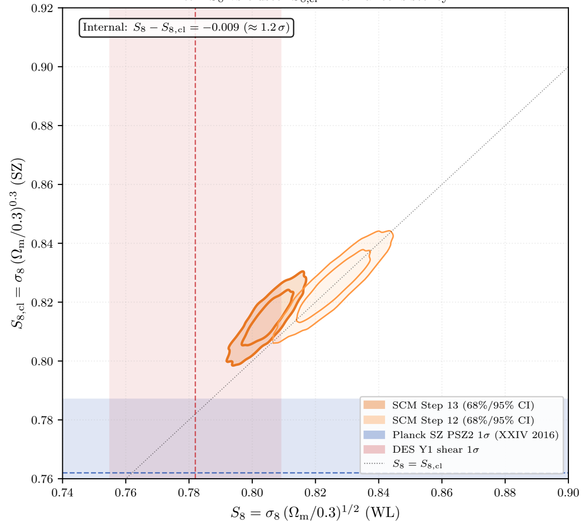
WL S_8 vs cluster S_{8,\text{cl}} : internal consistency
