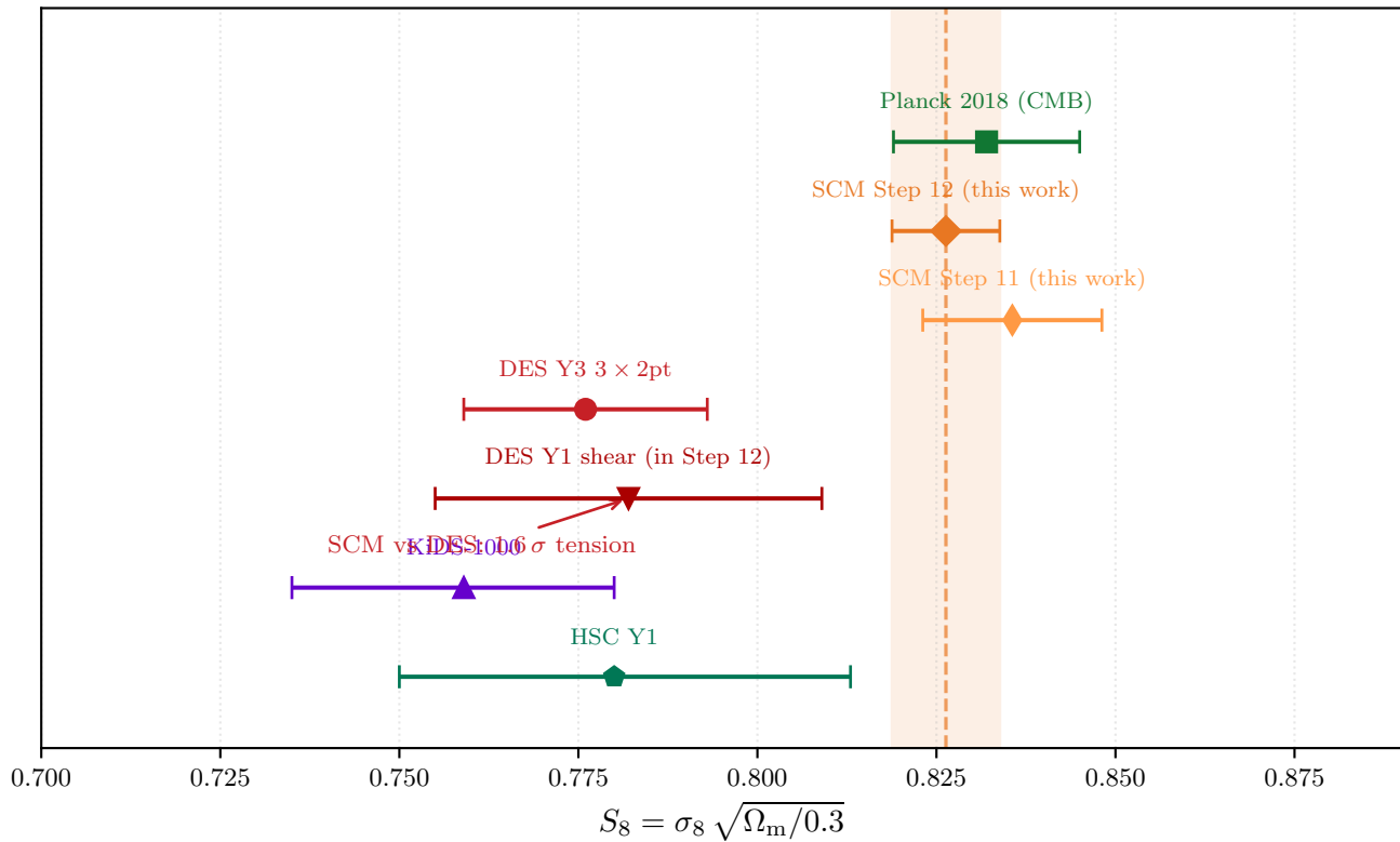
S_8 comparison: SCM Step 12 and weak-lensing surveys
