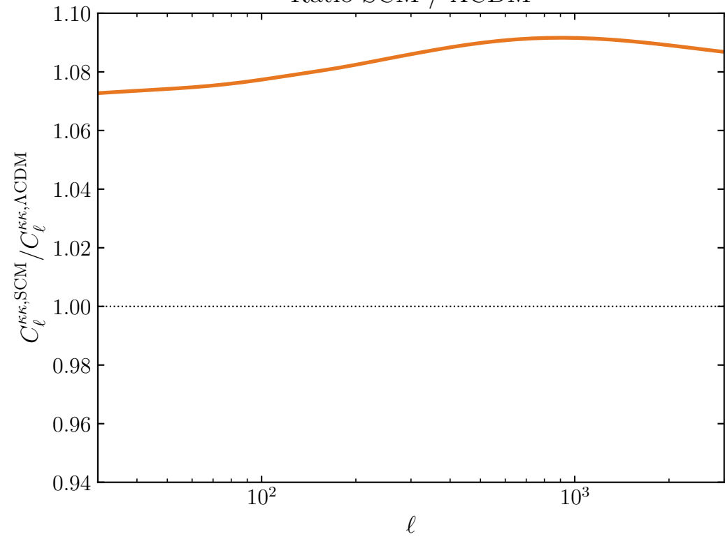
Ratio SCM / \Lambda CDM
