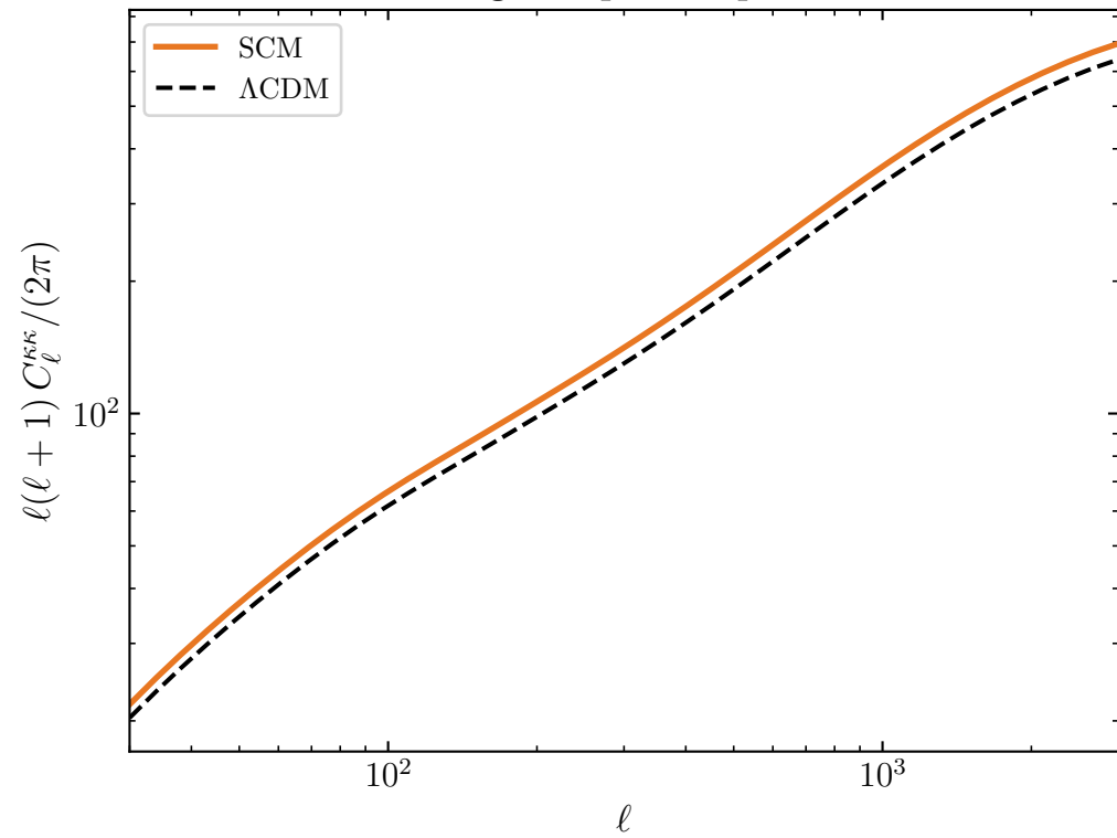
Convergence power spectrum
