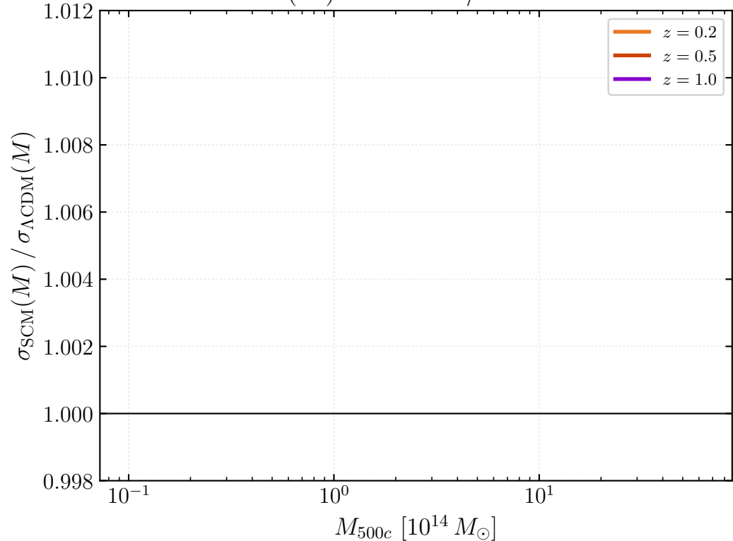
\sigma(M) ratio SCM/ \Lambda CDM
