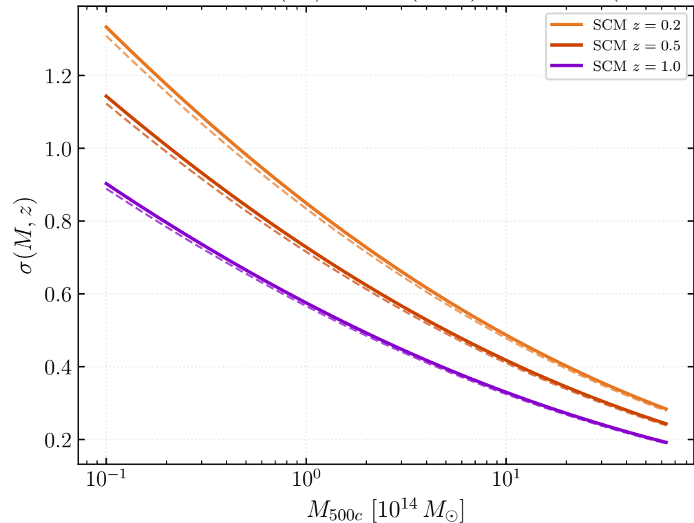
RMS fluctuation \sigma(M) : SCM (solid) vs \Lambda CDM (dashed)
