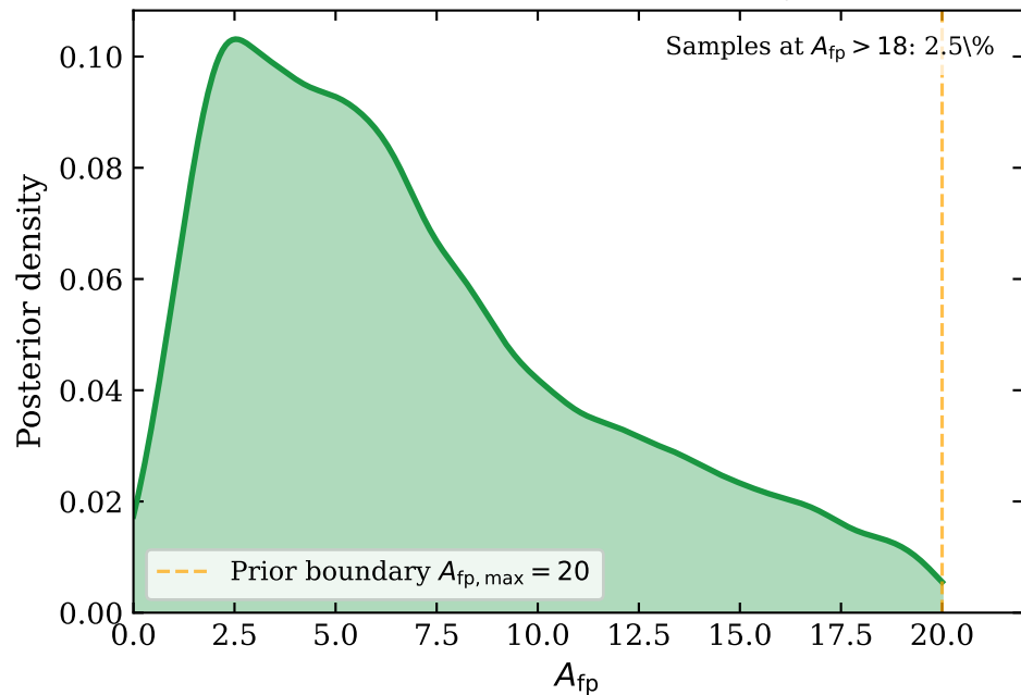
Step 10: A_{fp} — prior not constraining (2.5% near upper boundary)
