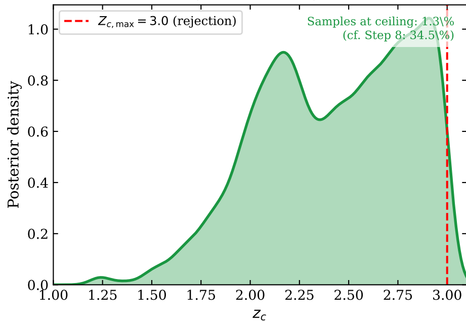
Step 10: z_c — no pileup at Z_{c, \max} (prior rejection correctly applied)
