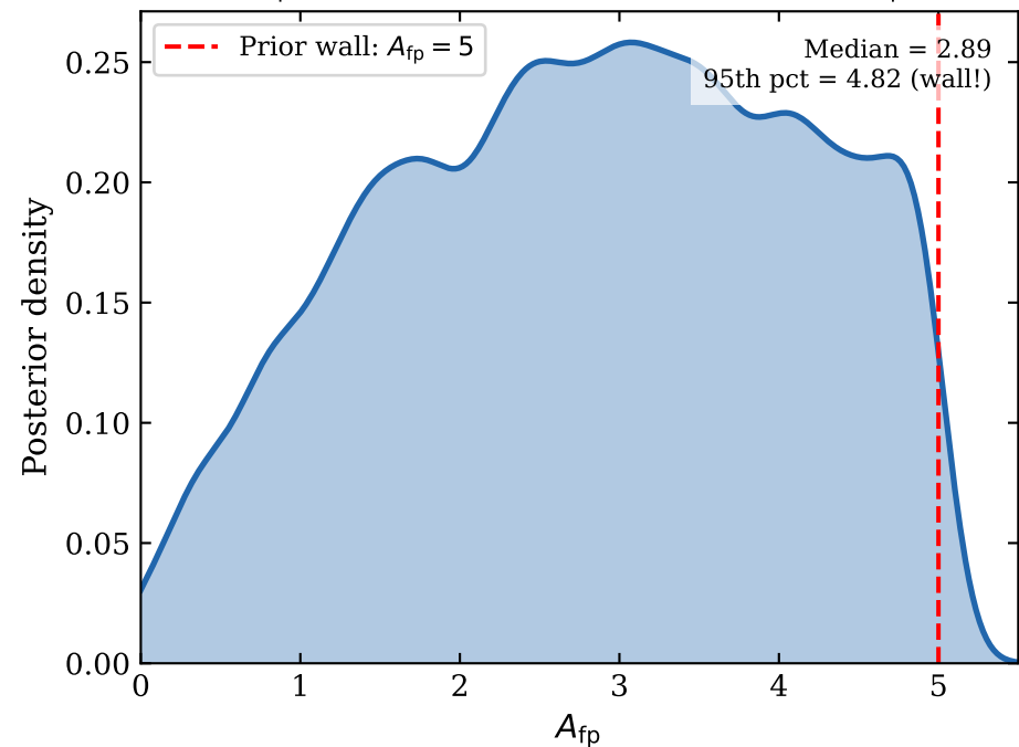
Step 7: A_{\text{fp}} posterior truncated at prior wall ( A_{\text{fp}, \text{max}} = 5 )
