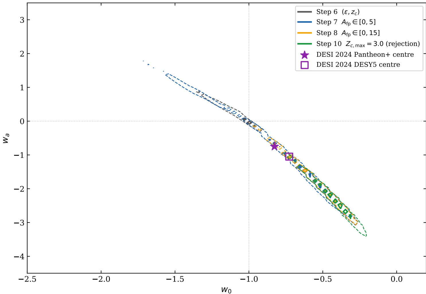
w_0 -- w_a plane: SCM Steps 6, 7, 8, 10 vs DESI 2024 (contours: 1\sigma and 2\sigma ; Step 9 excluded — not converged)
