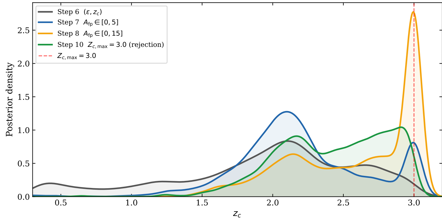
z_c posterior: Steps 6, 7, 8, 10 (Step 9 excluded — not converged, bimodal)
