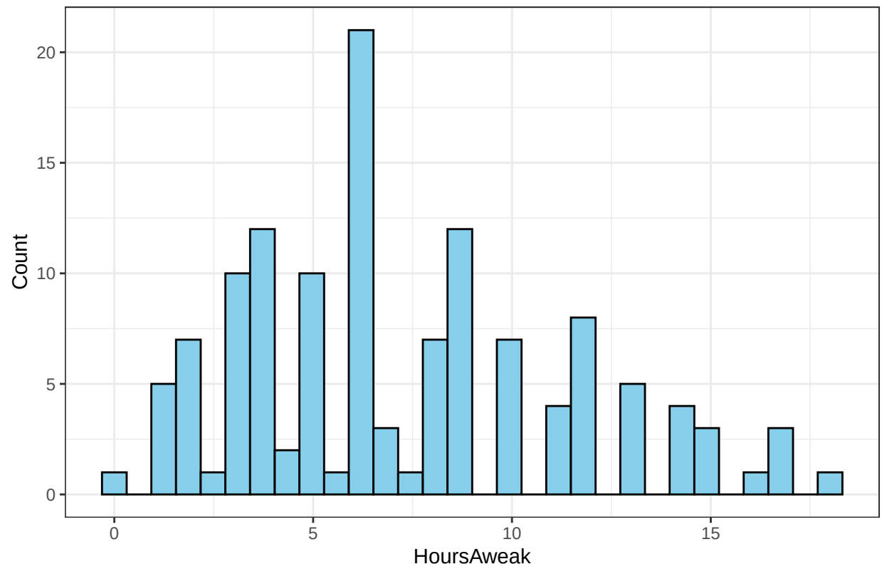
Histogram of HoursAweek
