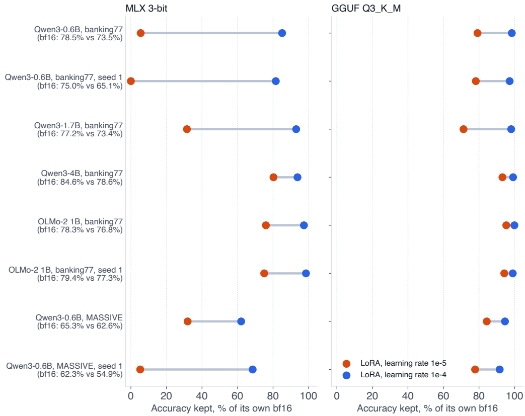
Figure 4: Accuracy kept, as a share of each model’s own bf16 accuracy, by the LoRA at 10^{-5} (orange) and the LoRA at 10^{-4} (blue), at MLX 3-bit and GGUF Q3_K_M, in all eight settings. Labels give the two bf16 accuracies. Exploratory.
