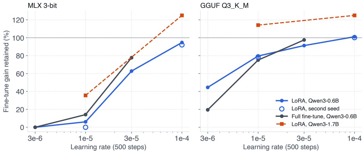
Figure 3: Gain retained at MLX 3-bit and GGUF Q3_K_M against learning rate. Qwen3-1.7B values above 125% are drawn at 125%, because its base collapses at 3 bits. Round 2, exploratory.
