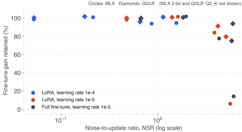
Figure 2: Gain retained against the noise-to-update ratio NSR (log scale) for the round-1 Qwen3-0.6B fine-tunes, at every format except MLX 2-bit and GGUF Q2_K. The base model also breaks at MLX 3-bit; the two points at the lower right are the gentle LoRA and the full fine-tune there. Circles: MLX; diamonds: GGUF.
