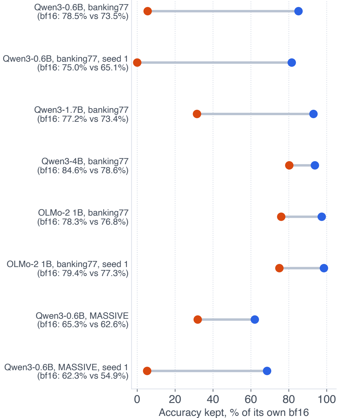
MLX 3-bit
