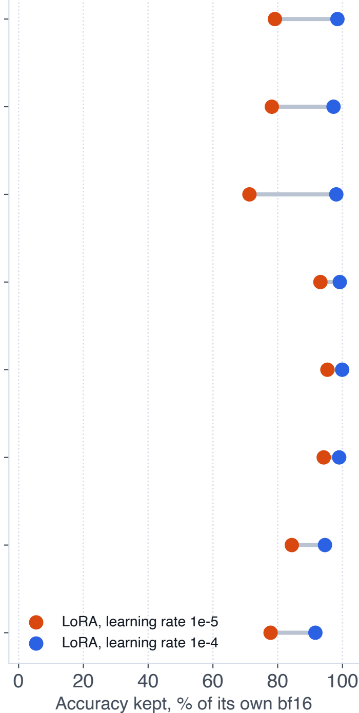
GGUF Q3_K_M
