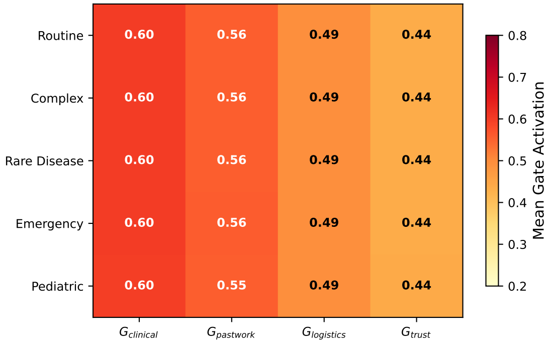
Context-Aware Gate Activations
