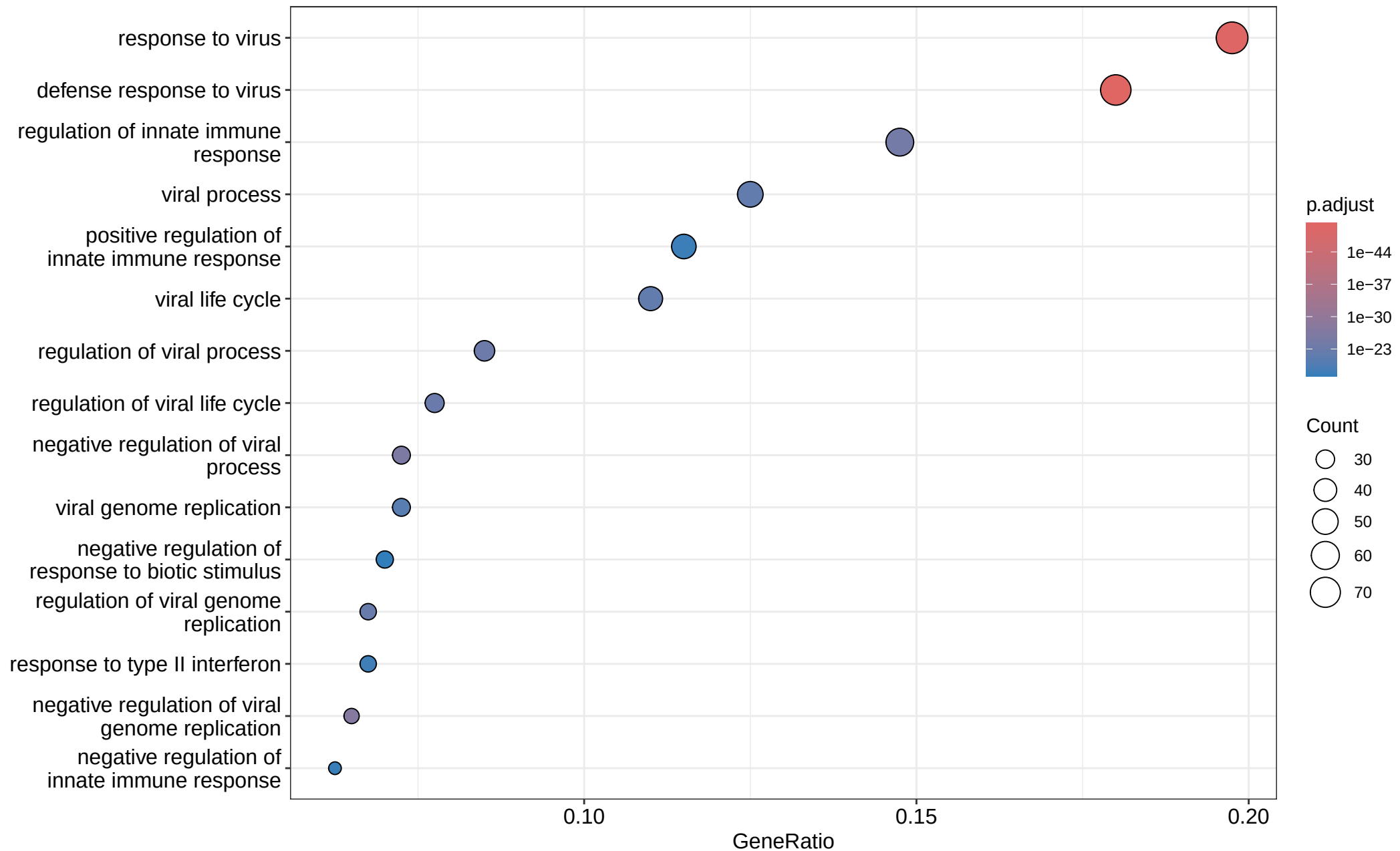
GO BP: ZIKV Positive vs Negative
