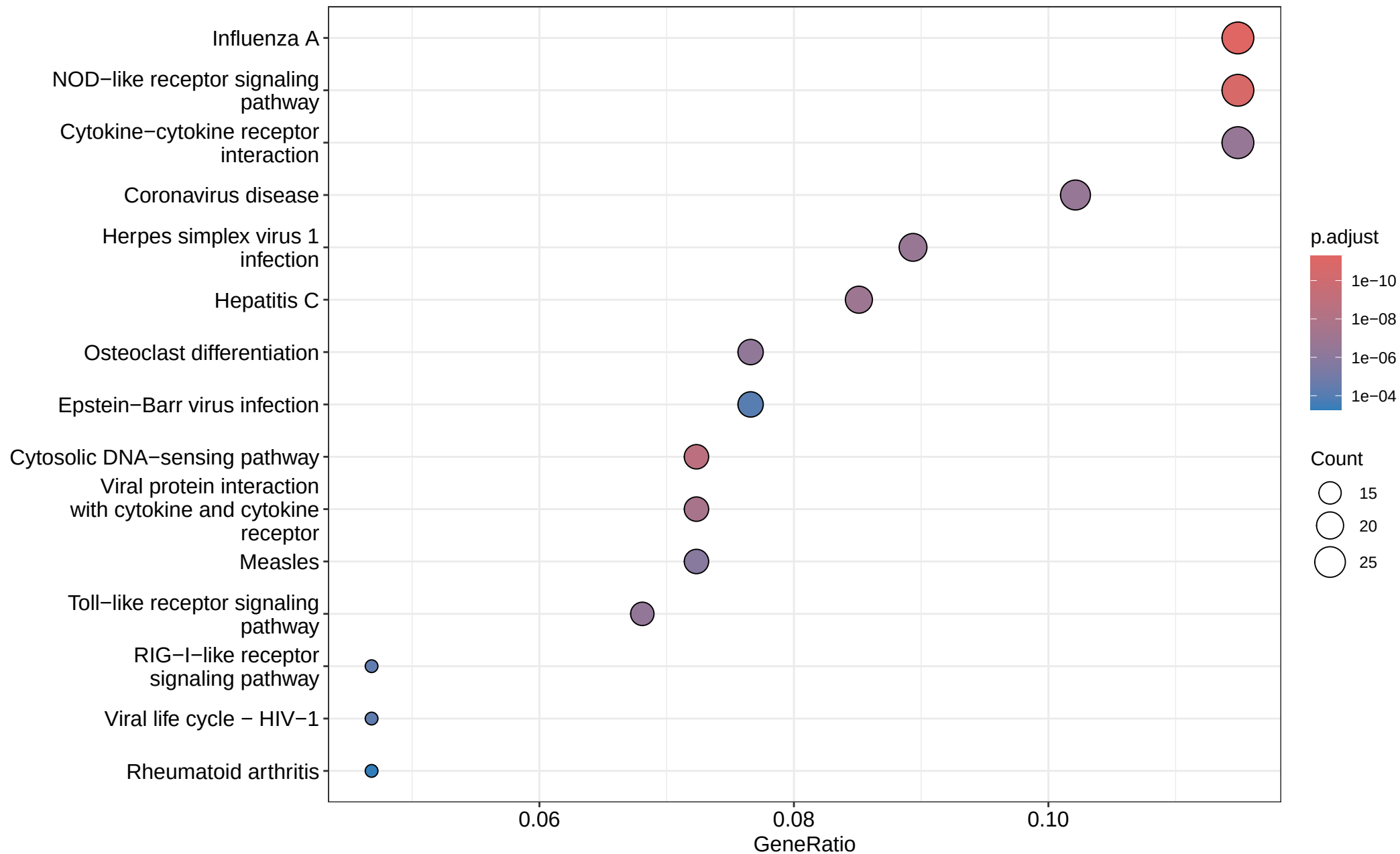
KEGG: ZIKV Positive vs Negative
