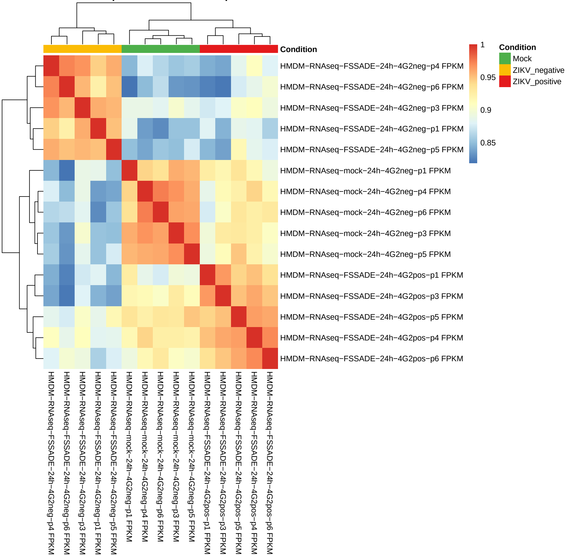
Sample Correlation Heatmap
