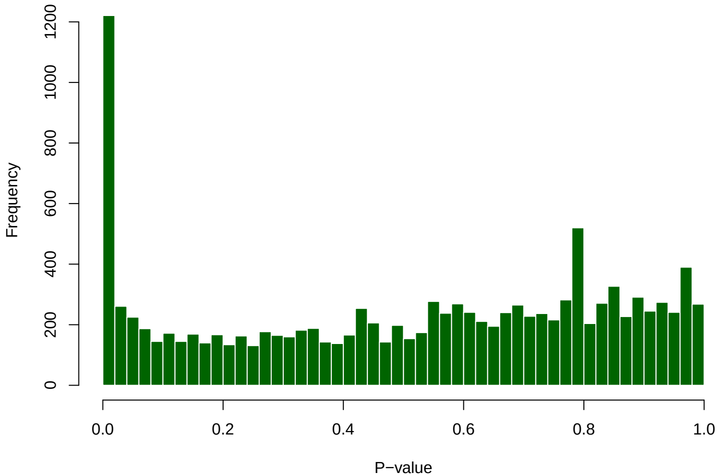
P-value Distribution: ZIKV_negative_vs_Mock
