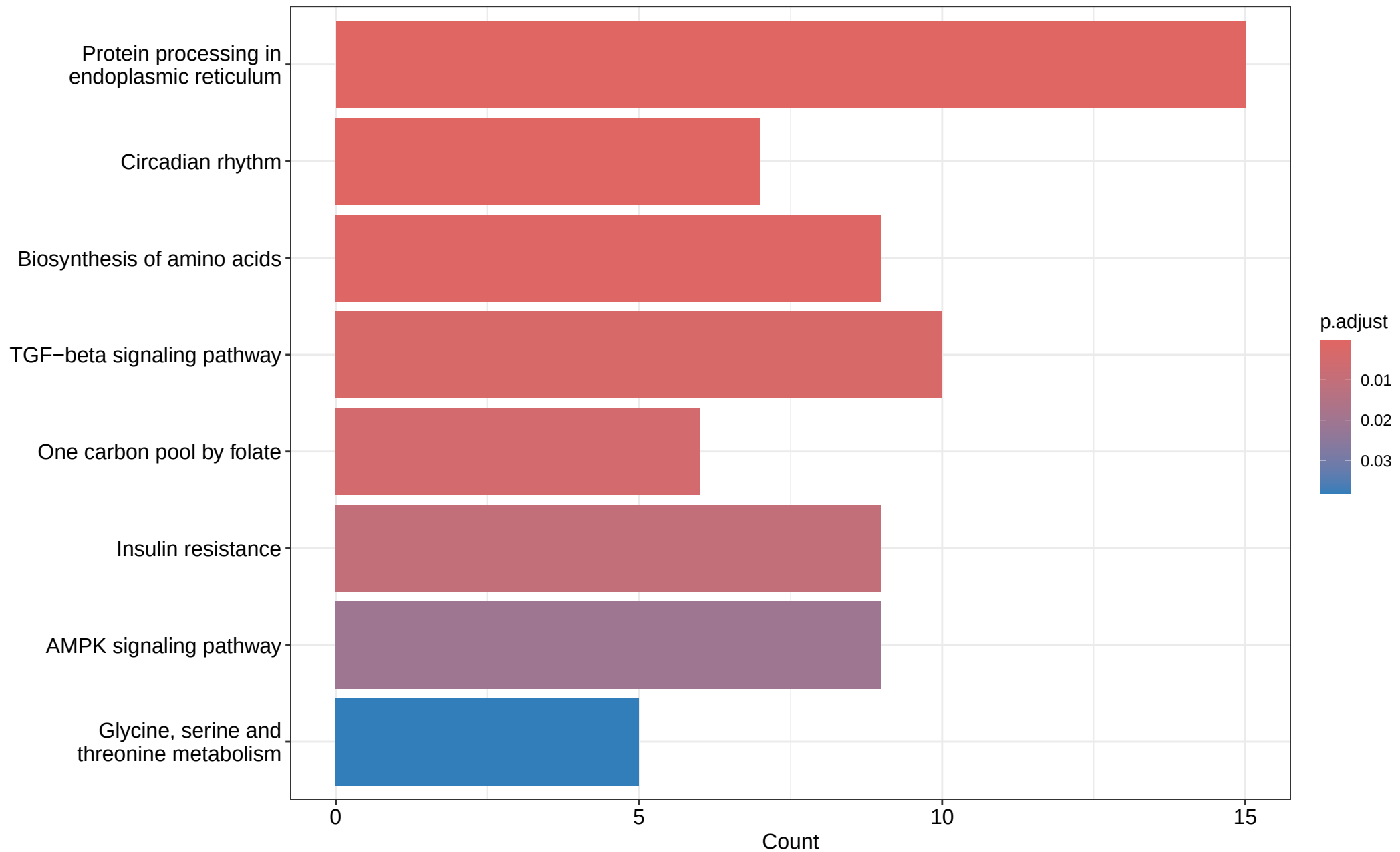
GSE78711_Up_in_ZIKV_DEG KEGG enrichment
