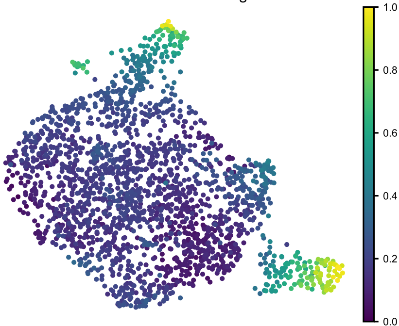
Pseudotime Ordering
