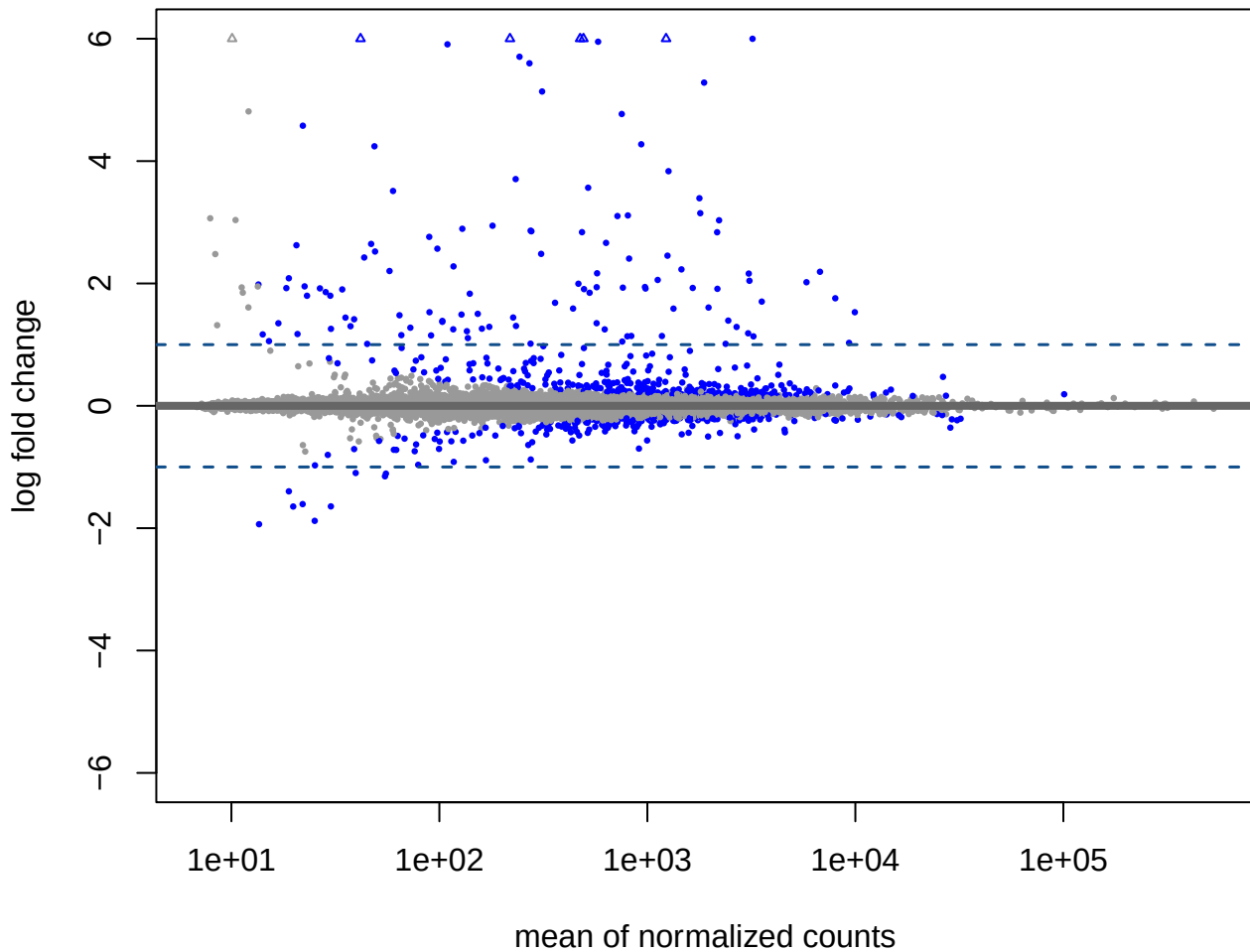
MA plot: ZIKV infected vs Control
