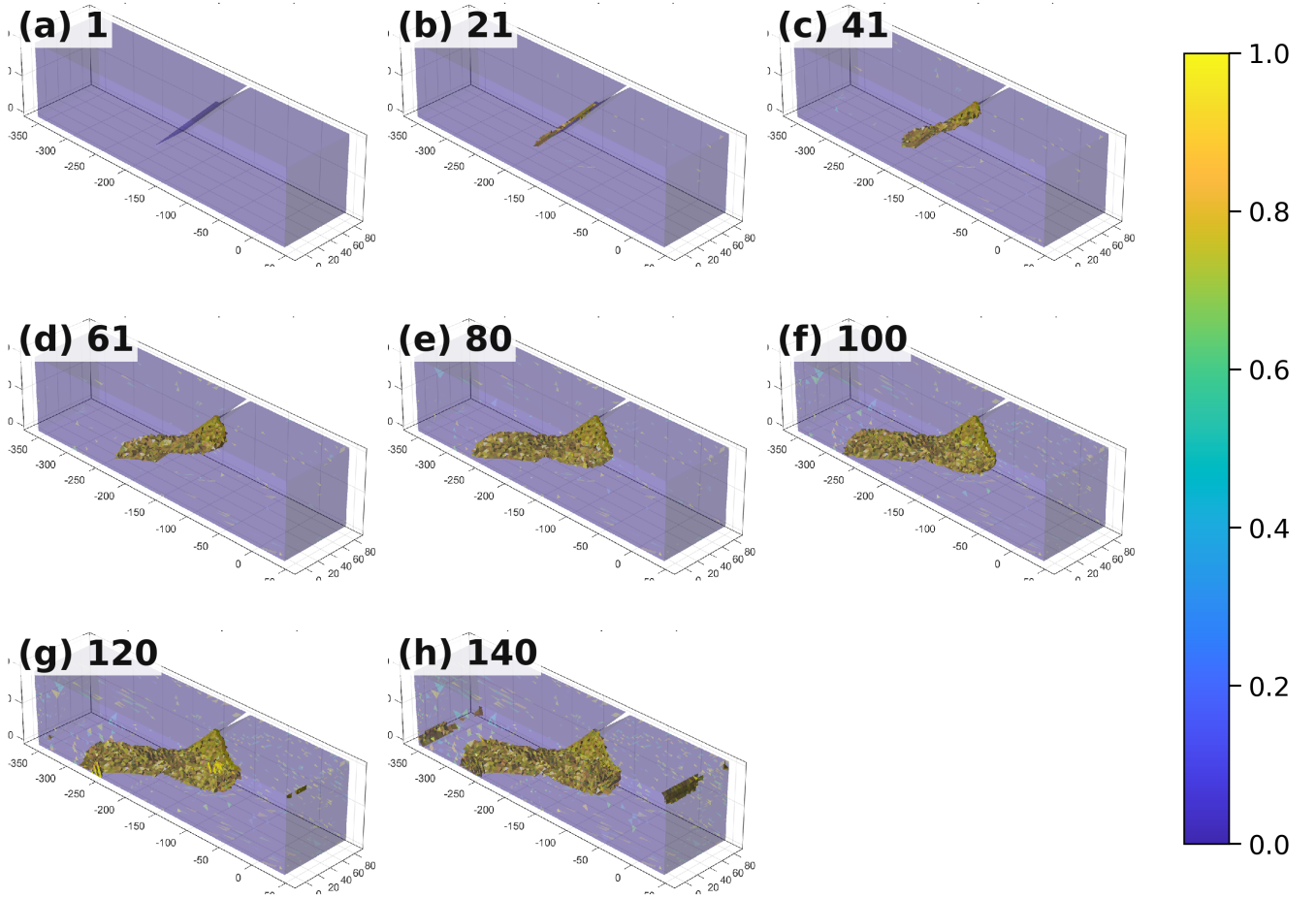
(b) Torsion damage sequence.
