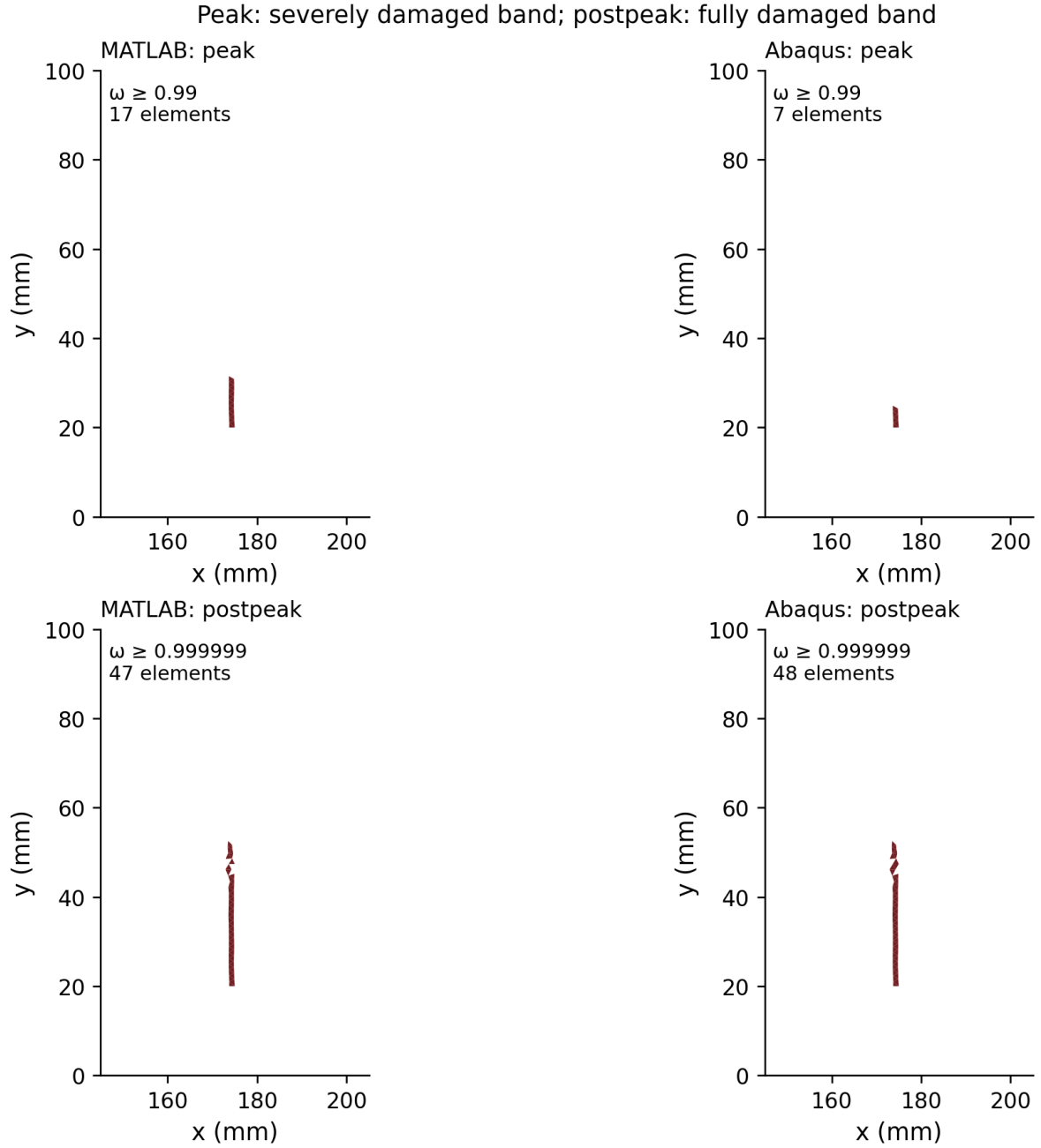
Figure 2: Damaged element bands in the notch region on the undeformed CPS3 mesh. Left: MATLAB; right: Abaqus/UMAT. Top: severe damage at peak load ( \omega \geq 0.99 ). Bottom: fully damaged elements ( \omega \geq 0.999999 ) after peak, at the saved state above CMOD 0.30 mm. The cutoffs differ between rows and are printed in each panel with the selected element count. These bands show damage localization, not a measured open-crack length. No smoothing is used. Abaqus uses the nearest stored response frame.
