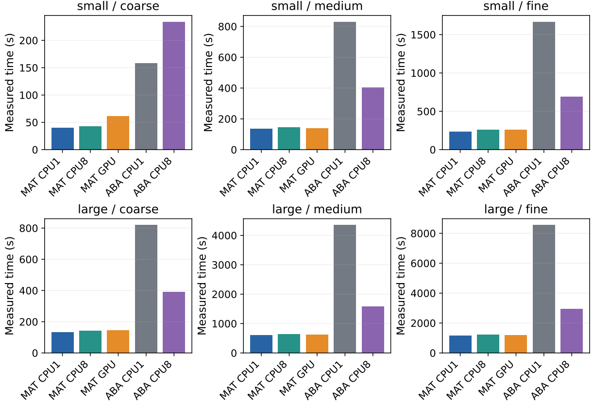
Figure 3: Thirty size/mesh/computing runs. MATLAB bars cover the load loop; Abaqus bars cover analysis and output. CPU8 denotes a MATLAB library-thread limit or Abaqus SMP; GPU denotes element/damage work with CPU sparse factorization. These workstation observations establish no cross-program speed ranking or GPU speed advantage.
