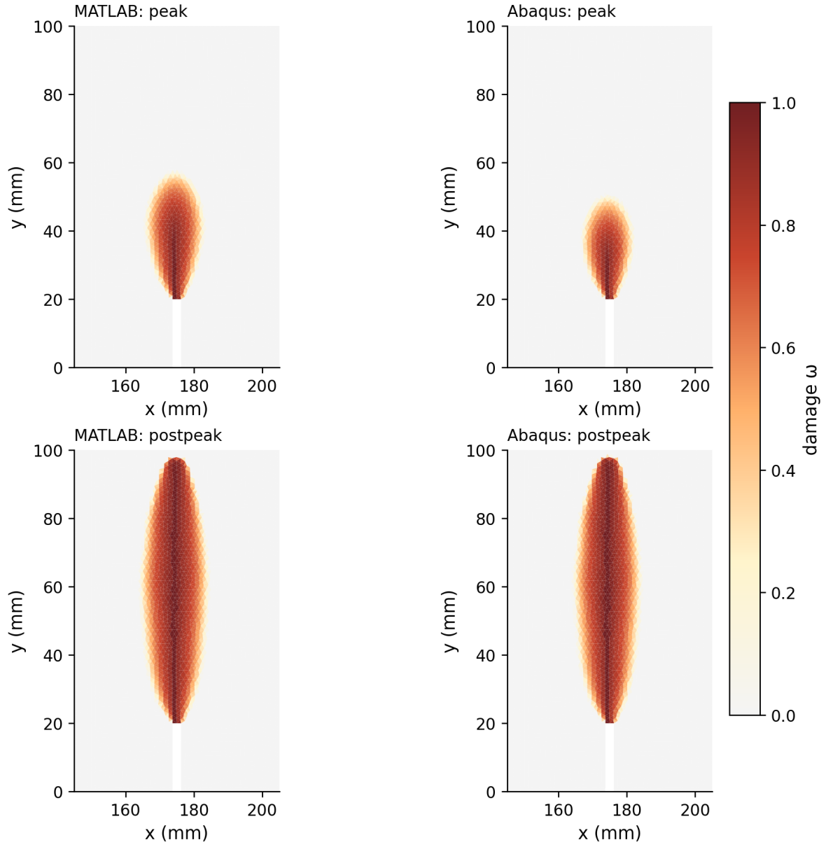
Figure 2: Damage field \omega in the notch region on the undeformed CPS3 mesh. Left: MATLAB; right: Abaqus/UMAT. Top: near peak load; bottom: post-peak state. Abaqus fields are the closest stored frames to the indicated response points.
