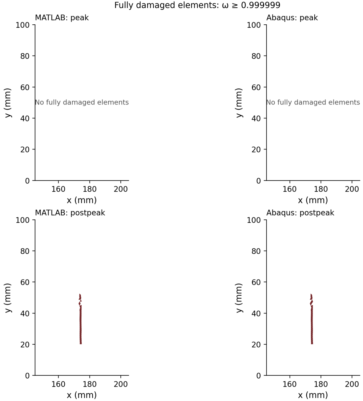
Figure 2: Fully damaged elements ( \omega \geq 0.999999 ) in the notch region on the undeformed CPS3 mesh. Partially damaged elements are omitted. Neither peak state contains elements at this cutoff, so the upper panels are empty. The lower panels show the computed element band, without smoothing or drawing an artificial crack line. Left: MATLAB; right: Abaqus/UMAT. Top: near peak load; bottom: post-peak state. Abaqus fields are the closest stored frames to the indicated response points.
