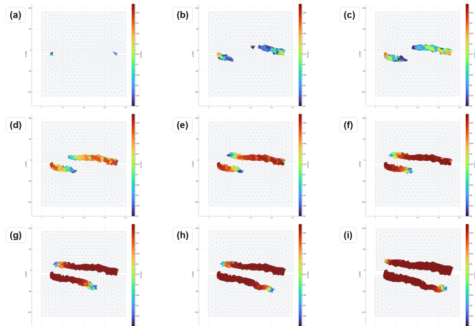
Figure 4: Nooru-Mohamed damage evolution from first localization to coalescence in a 3-by-3 sequence.
