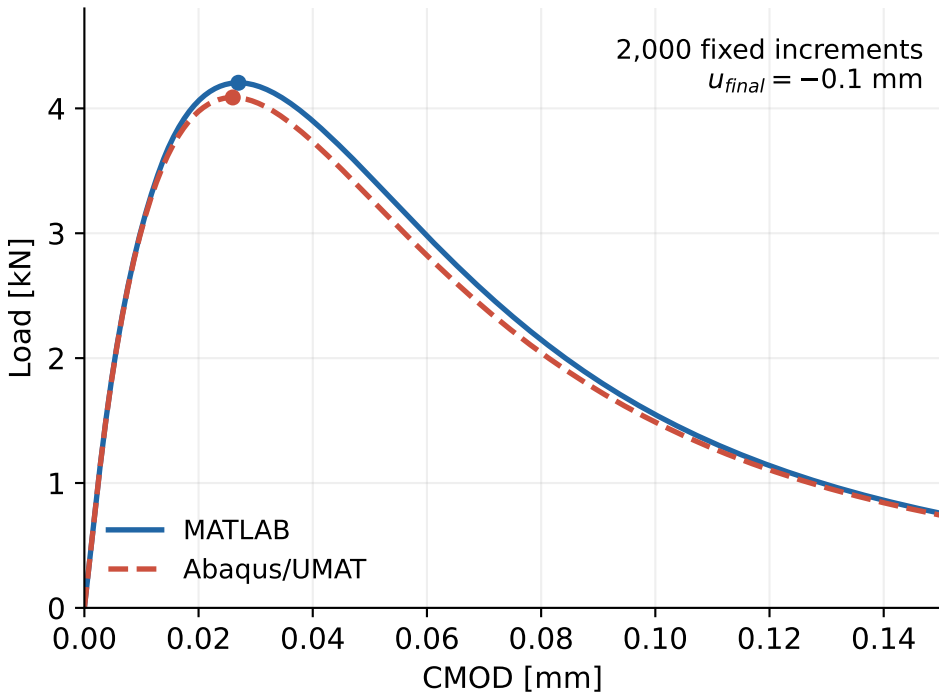
(b) Medium mesh
