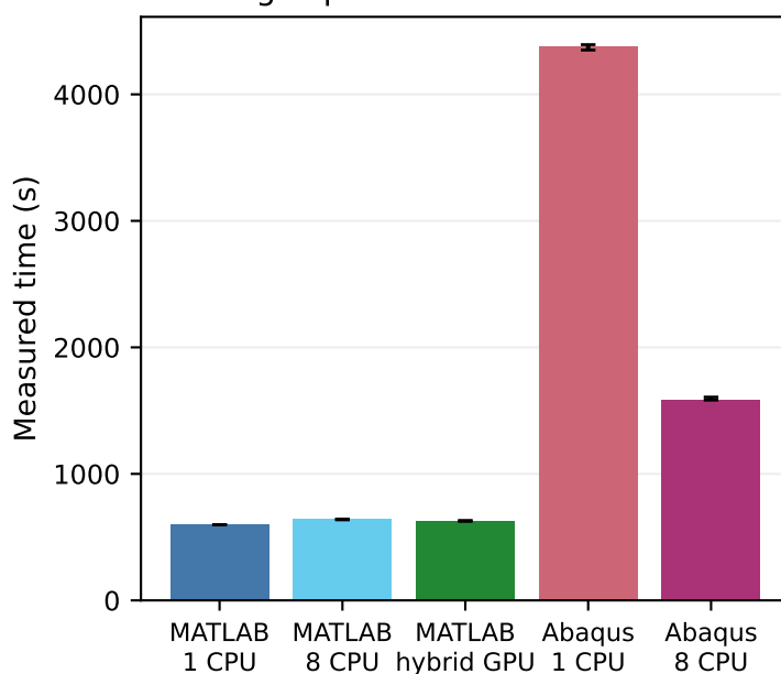
Large specimen - medium mesh
