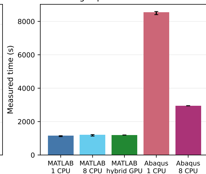
Large specimen - fine mesh
