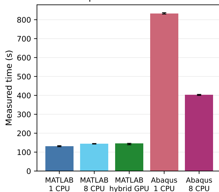
Large specimen - medium mesh
