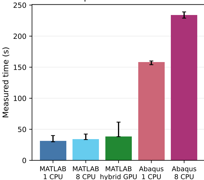
Large specimen - coarse mesh
