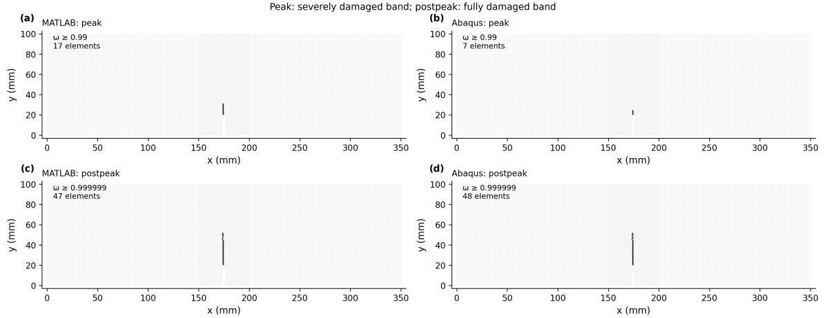
Figure 2: Damaged element bands on the full undeformed beam. The light grey background shows the CPS3 mesh; dark elements meet the displayed cutoff. Left: MATLAB; right: Abaqus/UMAT. Top: severe damage at peak load ( \omega \geq 0.99 ). Bottom: fully damaged elements ( \omega \geq 0.999999 ) after peak, at the saved state above CMOD 0.30 mm. The cutoffs differ between rows and are printed in each panel with the selected element count. These bands show damage localization, not a measured open-crack length. No smoothing is used. Abaqus uses the nearest stored response frame.
