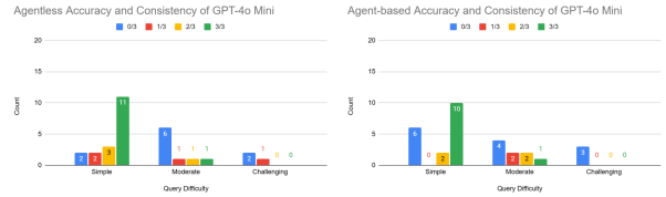
(b) Accuracy and Consistency of GPT-4o mini
