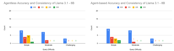
(c) Accuracy and Consistency of Llama 3.1 8B
