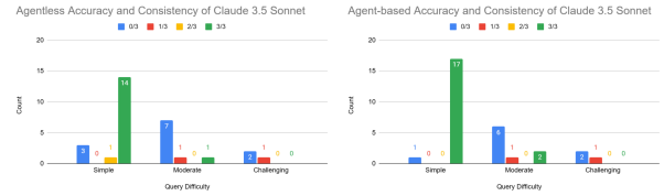
(a) Accuracy and Consistency of Claude 3.5 Sonnet
