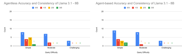
(c) Accuracy and Consistency of Llama 3.1 8B
