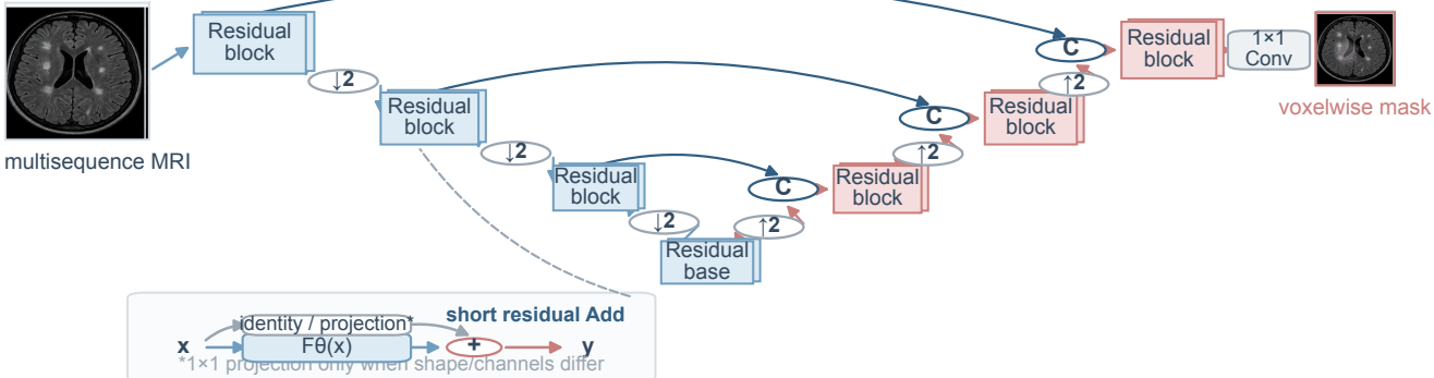
(c) Residual U-Net
