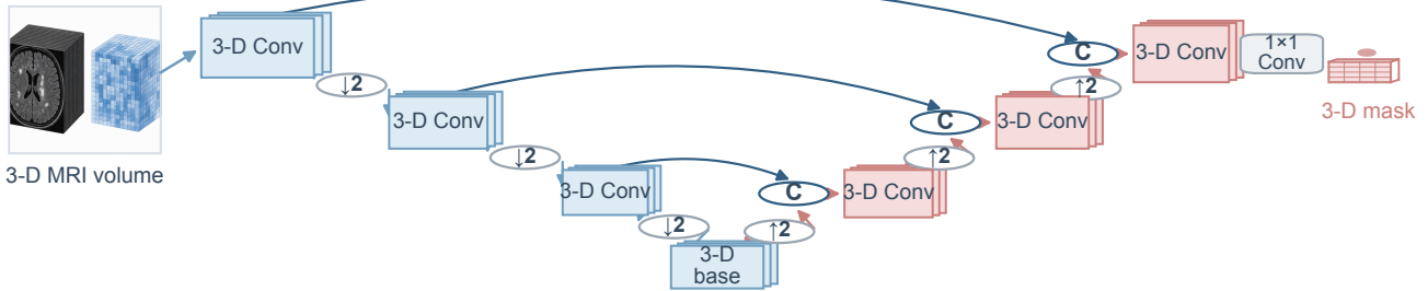
(b) 3D U-Net
