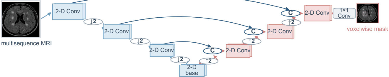
(a) U-Net
