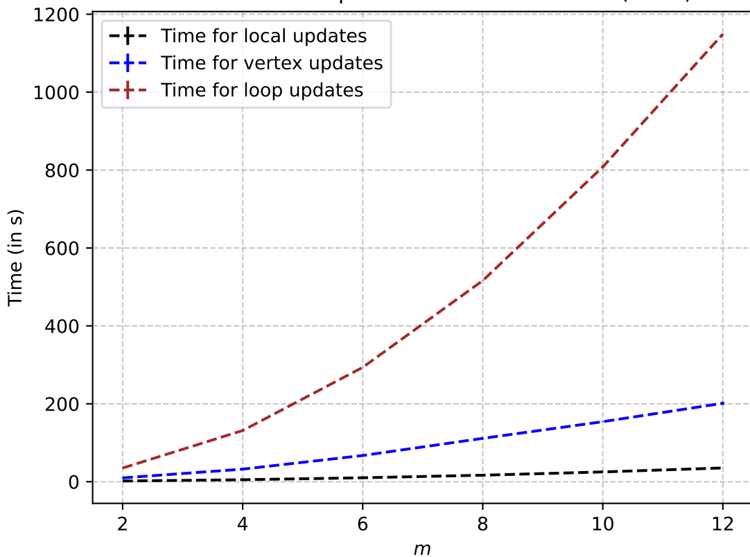
Time of one computation in function of m ( n = 8 )
