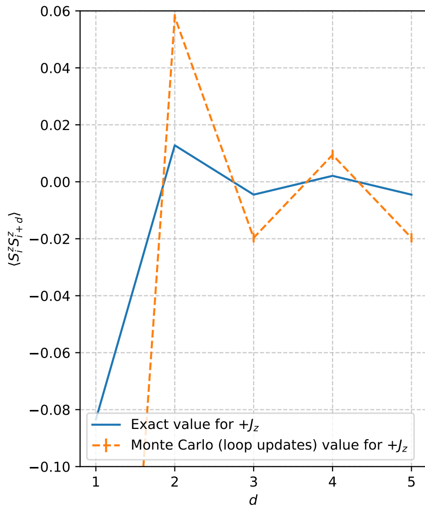
Spin correlation for n = 8, J_x = 2.2, J_z = \pm 1, T = 1, m = 6
