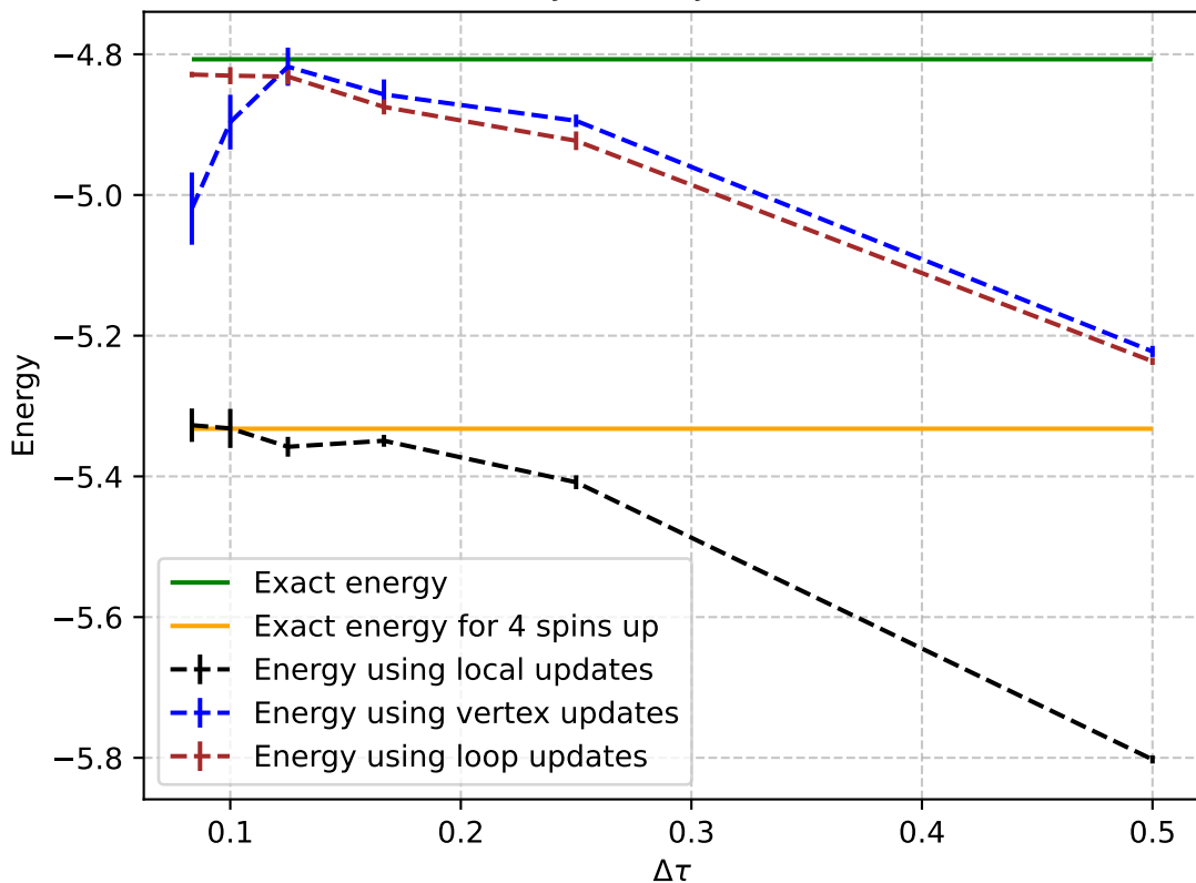
Energy in function of \Delta\tau n = 8, J_x = 2.2, J_z = 1, T = 1
