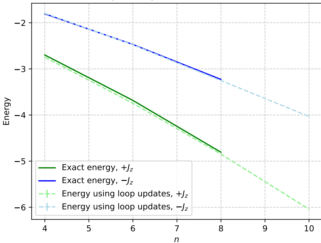
Energy in function of n and \pm J_z J_x = 2.2, J_z = 1, T = 1, m = 6
