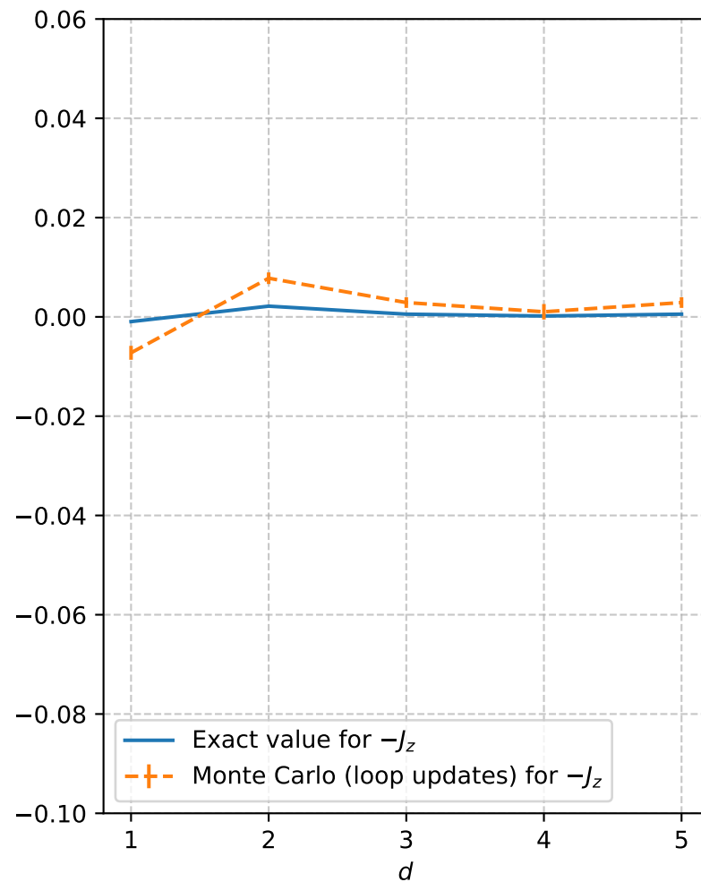
Spin correlation for n = 8, J_x = 2.2, J_z = \pm 1, T = 1, m = 6
