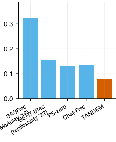
NDCG@10
