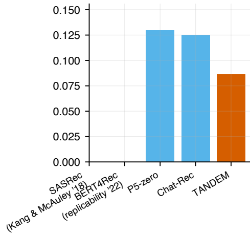
MRR
