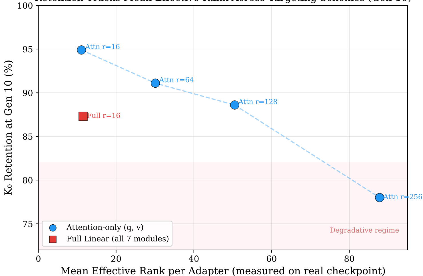
Retention Tracks Mean Effective Rank Across Targeting Schemes (Gen 10)
