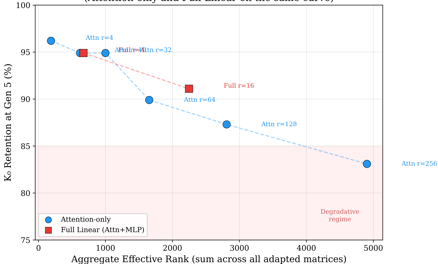
Retention vs Aggregate Effective Rank (Attention-only and Full-Linear on the same curve)
