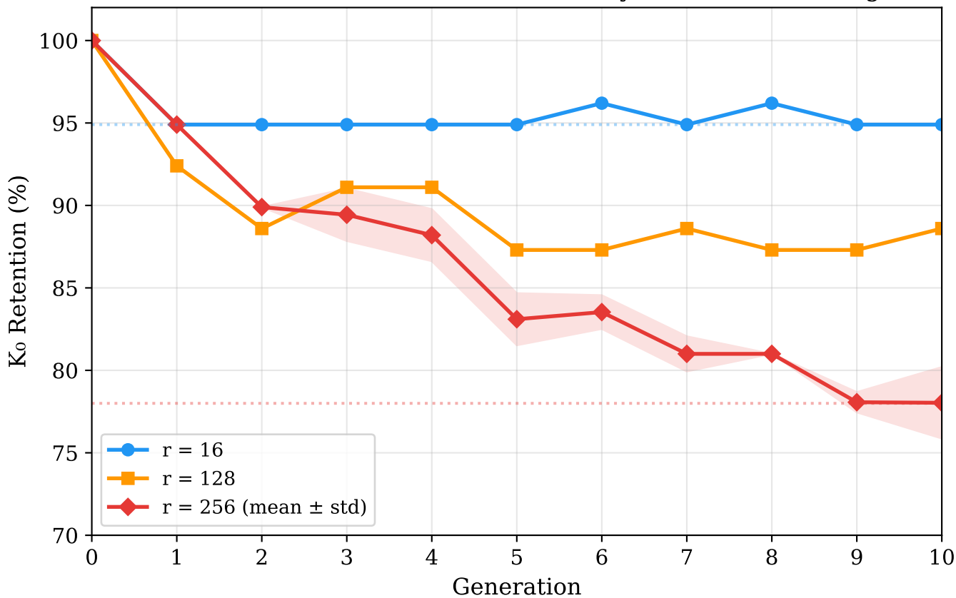
Factual Retention Under Recursive Synthetic Fine-Tuning
