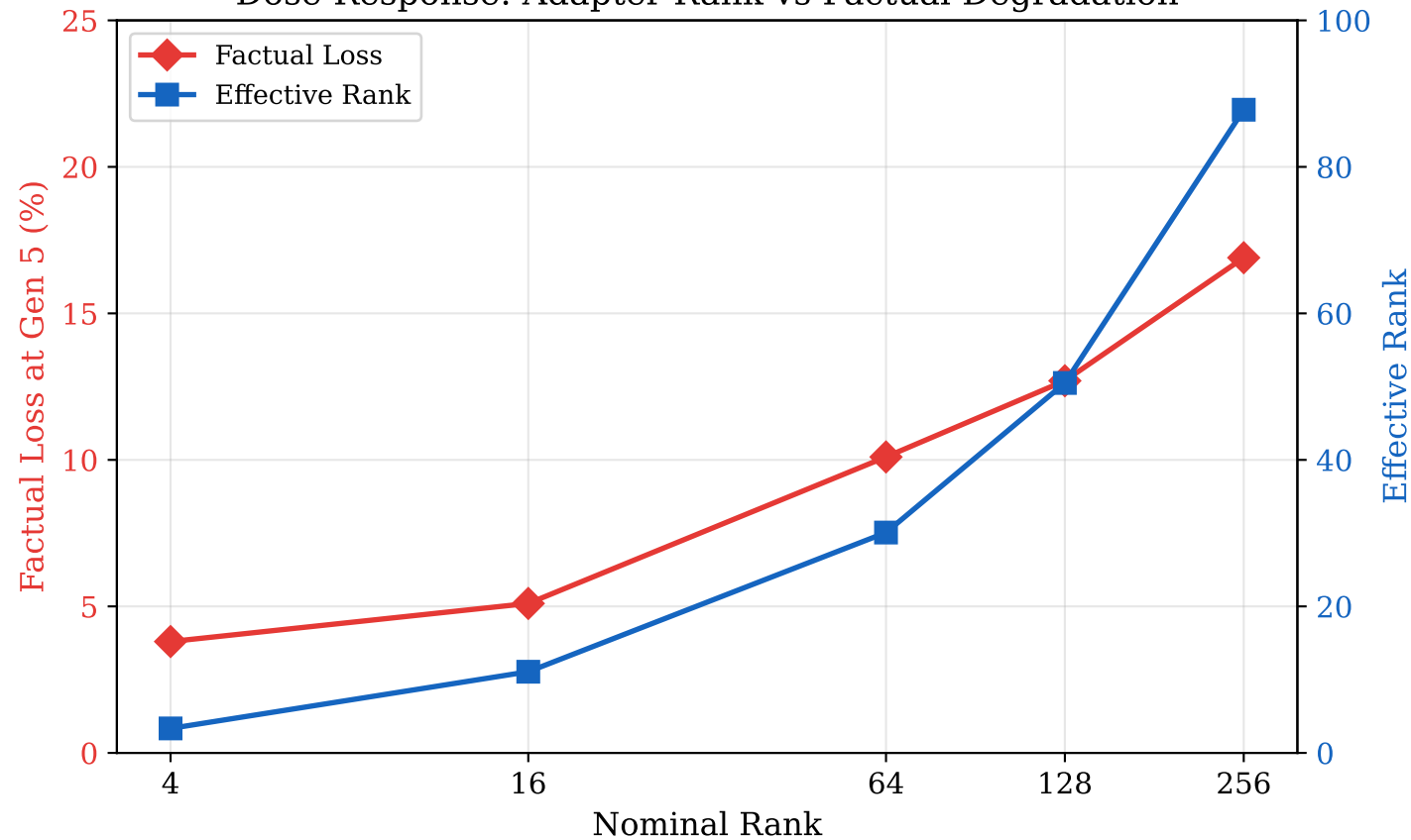
Dose-Response: Adapter Rank vs Factual Degradation
